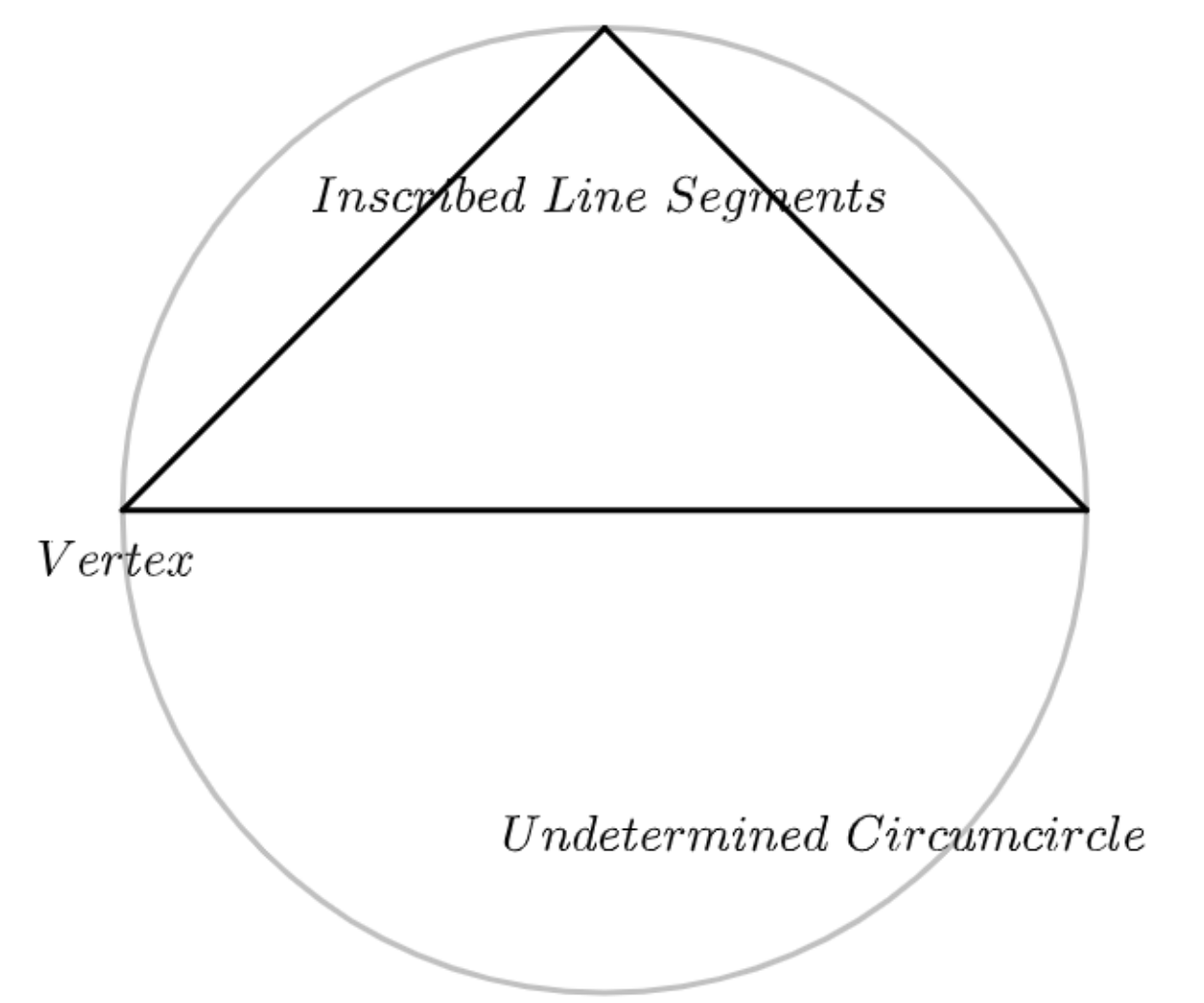
Three Inscribed Lines Three Vertices Trigonometry
