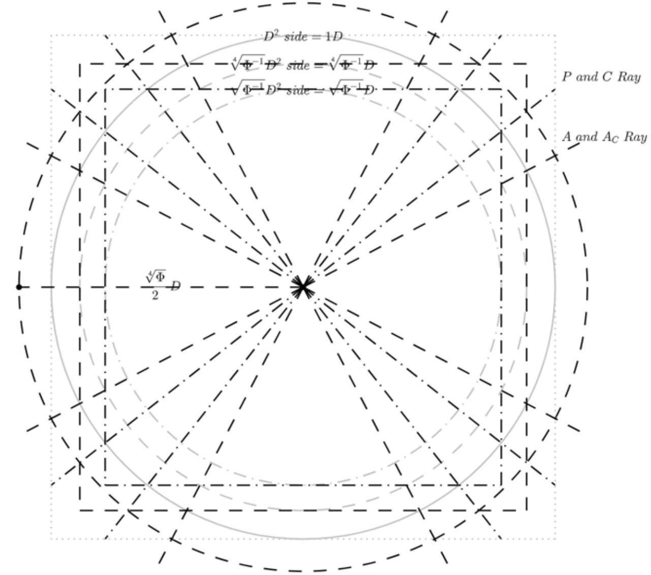
Inscribe Smaller "O"s in "□"s, Radial Angles for Square Circled
